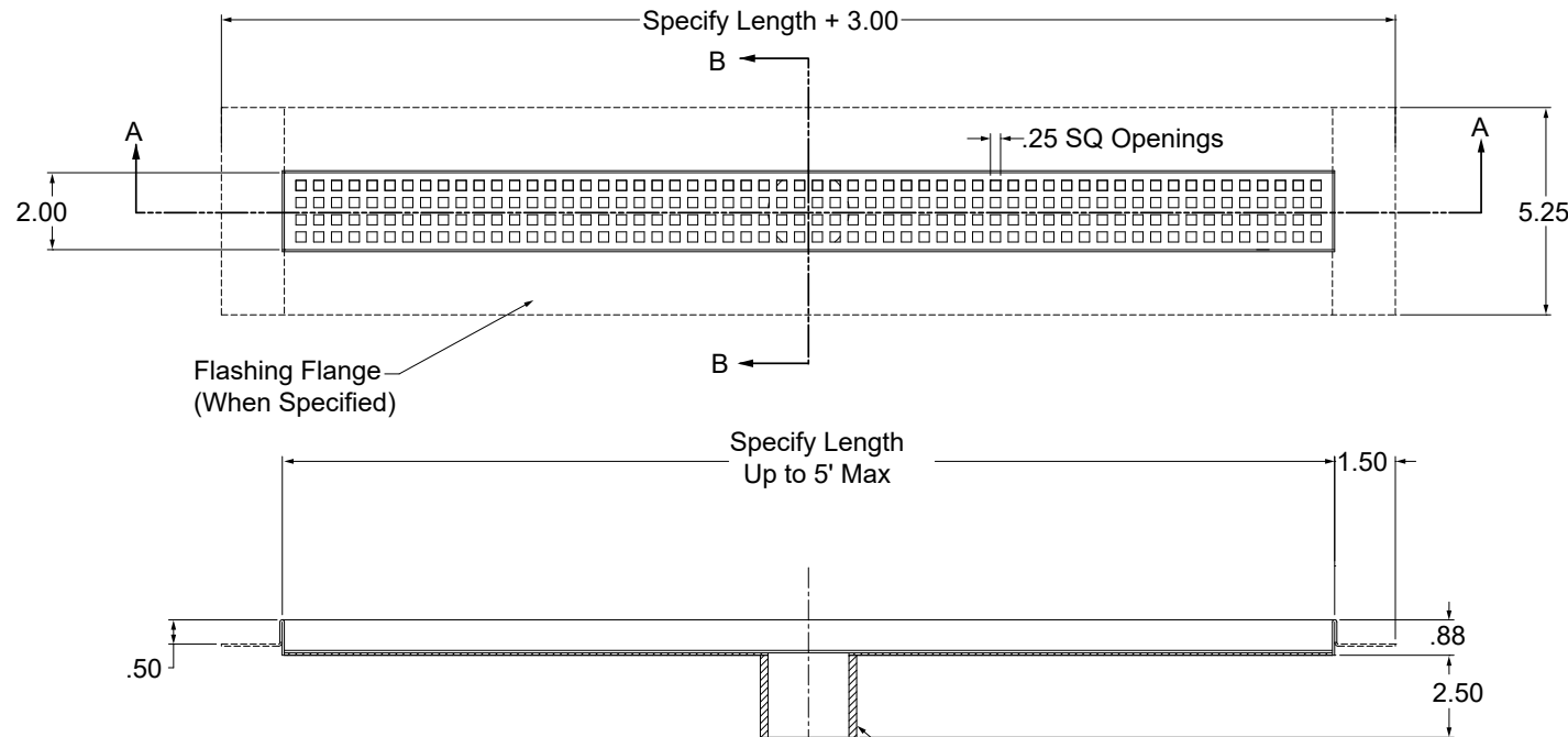
SECTION A-A — 2" NO-HUB Outlet
