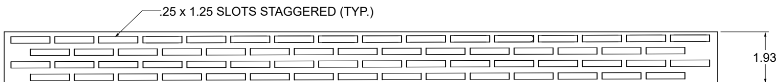
SLOTTED GRATE -SLG
